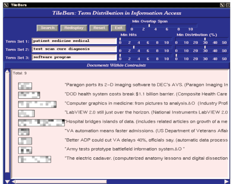
Figure 5. (Case 15) TileBar search on (patient medicine medical AND test scan cure diagnosis AND software program) with stricter distribution constraints.
